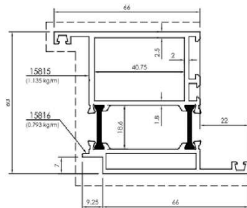
20213 (1.928 kg/m) (THERMAL BIG Z)
