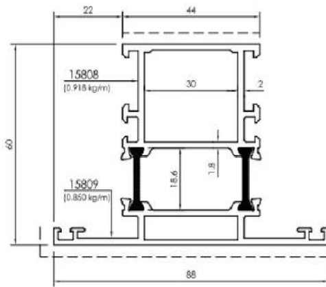
20214 (1.768 kg/m) (THERMAL BIG T)
