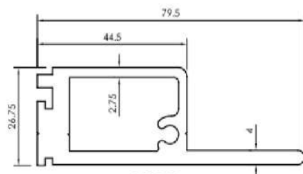
12871 (1.797 kg/m) TO JOIN T-PROFILE WITH THE FRAME PROFILES-20204, 20211 & TO THE SASH PROFILE 20213 (MILL FINISH)
