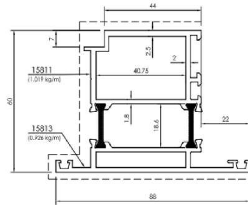
20212 (1.945 kg/m) (THERMAL BIG T OPEN OUT)
