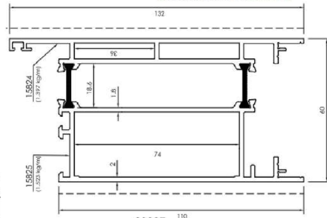
20227 (2.920 kg/m) (12CM TH. HING BOTTOM)
