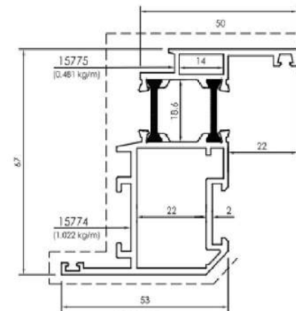
20207 (1.503 kg/m) (THERMAL SMALL Z)
