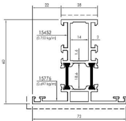
20208 (1.449 kg/m) (THERMAL SMALL T)
